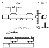
Single lever shower mixer Anti-limescale hand shower with directable support. Shower hose satin (91.34.609.15).
