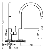
Monocomando lavello verticale MAX Single lever single hole sink mixer MAX Jedn3p3kov3 dřeřov3 kuchyŇisk3 baterie MAX
