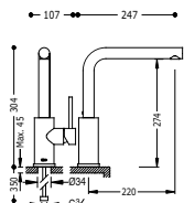
Monocomando lavello verticale MAX Single lever single hole sink mixer MAX Jedn3p3kov3 dřeřov3 kuchyŇisk3 baterie MAX
