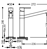
Monocomando lavello verticale LEX-TRES canna lunga Single lever single hole sink mixer LEX-TRES tube spout Jednopáková dřezová kuchyňská baterie LEX-TRES dlouhé ramínko
