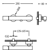
Single lever shower mixer Anti-limescale hand shower with directable support. Shower hose satin (91.34.609.15).
