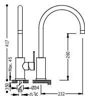
Monocomando lavello verticale LEX-TRES Single lever single hole sink mixer LEX-TRES Jednopáková dřezová kuchyňská baterie LEX-TRES
