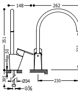
Monocomando lavello verticale LEX-TRES Single lever single hole sink mixer LEX-TRES Jednopáková dřezová kuchyňská baterie LEX-TRES
