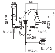
Accumulatore lavabo Wash-basin mixer Umyvadlová baterie
