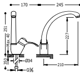
Monocomandoavello verticale MONOCLASIC-1900 Single lever single hole sink mixer MONOCLASIC-1900 Jednopaková dřezová kuchyňská baterie MONOCLASIC-1900
