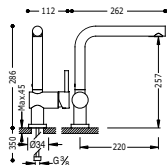
Monocomando lavello verticale Single lever single hole sink mixer Jedn3p3kov3 dřeřov3 kuchyŇisk3 baterie
