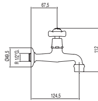
Rubinetto office Kitchenette tap Kuchyňská baterie
