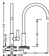
Monocomando lavello verticale CLASS Single lever single hole sink mixer CLASS Jedn3p3kov3 dřeřov3 kuchyŇisk3 baterie CLASS
